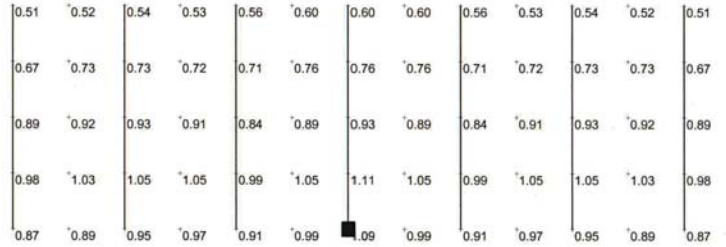
60' x 60' spacing 20'MH AVG. FC=.70; 3.8 to 1 max to min
