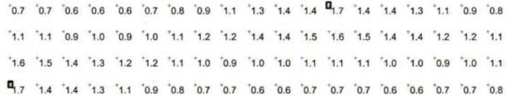
60' x 60' spacing 20'MH AVG. FC=.70; 3.8 to 1 max to min
